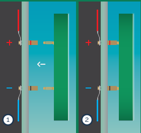
Banana Plugs
